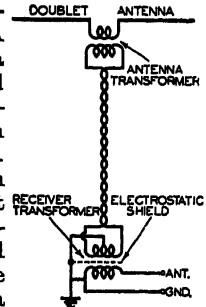
Noise-reducing antenna circuit.
